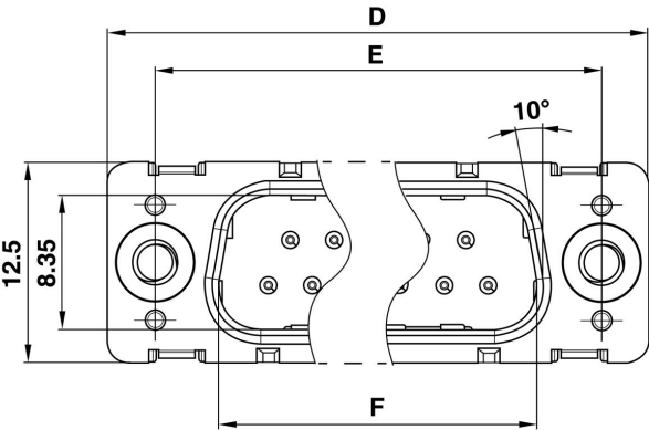
Plug
